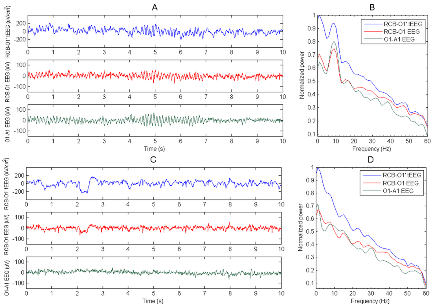
Fig. 3. Global physiological rhythms such as alpha activity observable with eyes closed can be recorded by TCRES. Panel A: the top trace (blue) is tEEG from a TCRE placed next to the conventional disc electrode at O1. The middle trace (red) is from the conventional disc electrode at O1. Both the top and middle traces are recorded with respect to the reference on the right collar bone (RCB). The bottom trace (green) is from the O1 electrode with respect to the A1 reference electrode. Panel B: the power spectral densities for the signals of panel A. Panels C and D are the signals and power spectral densities when the eyes are open. It is evident that the alpha waves are present in both tEEG and EEG records, specifically between 4 and 5 seconds (panel A), which is confirmed by the spectra displaying a peak just below 10 Hz (panel B) but are not seen in panels C and D.
