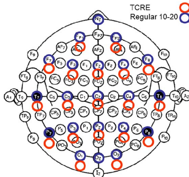
Fig. 2. The 10-5 montage with TCREs (red) placed near the 10-20 locations. Note: T7/P7 and T8/P8 are the same as T3/T5 and T4/T6 in 10-20 nomenclature. The blue rings are for standard 10-20 electrode locations.
