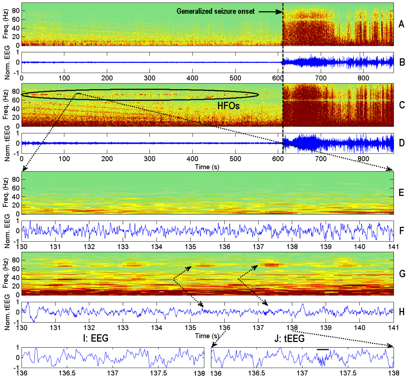
Fig. 5. A representative example of simultaneously recorded EEG and tEEG from one patient. Conventional EEG (bipolar montage, channel F8-F4, panels B, F and I, 1-70 Hz, 200 S/s), tEEG (from a tripolar electrode placed right behind the F8 position (F8'), panels D, H and J, 1-100 Hz, 200 S/s), and their spectrograms (panels A, E and panels C, G for EEG and tEEG, respectively) starting ~10 min before and continuing during a generalized seizure with onset marked with the dashed vertical black line. The seizure is identified by marked increases in signal amplitude and power at all frequencies. Panels E-H: eleven-second EEG and tEEG segments (marked by the black line in panel C) are shown at higher temporal resolution. Note a series of high gamma-band burst HFOs at 60-80 Hz (highlighted by ellipse in C) occurring about every 2 s, which are clearly seen in the tEEG spectrogram only. Panels I, J: Further zoom-in of two-second segment shows one HFO in tEEG (black horizontal line in the panel J) while this HFO is absent in EEG (panel I).
